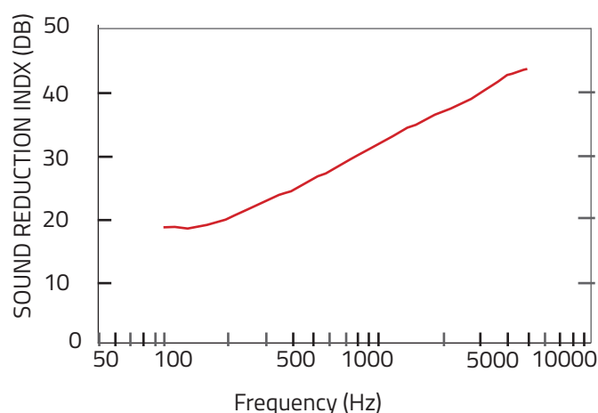
Bs En Iso10140-2 Free Hanging curtain RW (C;Ctr)=31 (-1;-4) dB
